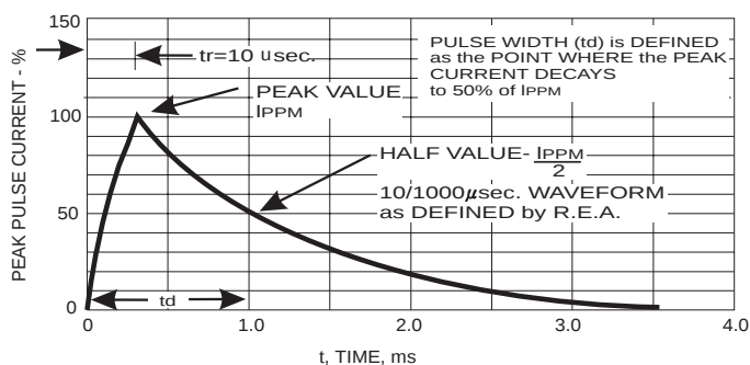
FIG.3- PULSE WAVEFORM
