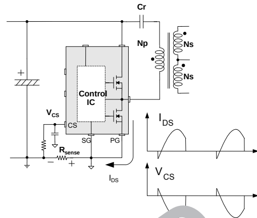
Figure 27. Half-Wave Sensing
