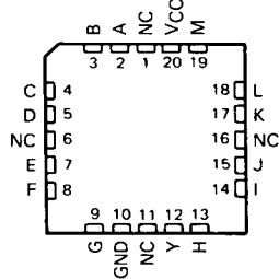
SN54HC133 . . . FK PACKAGE
