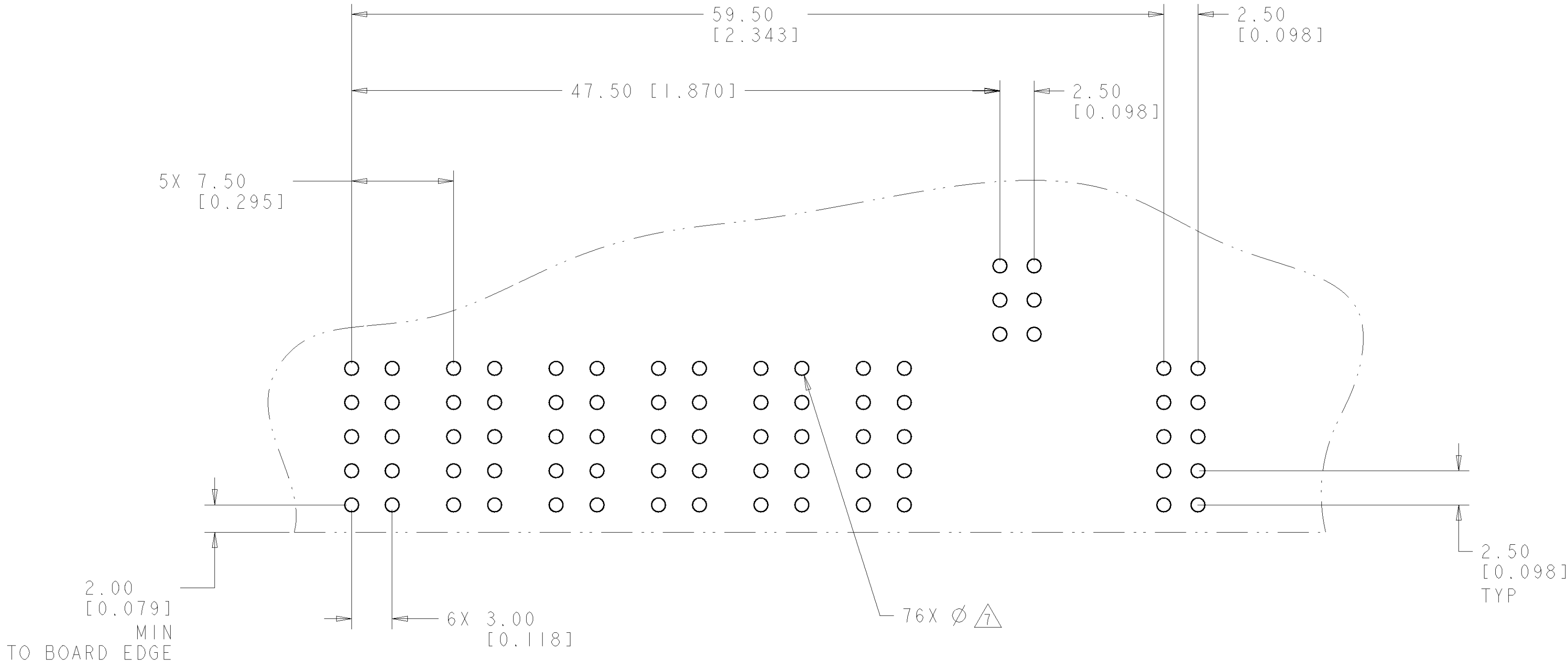
PRINTED CIRCUIT LAYOUT COMPONENT SIDE
