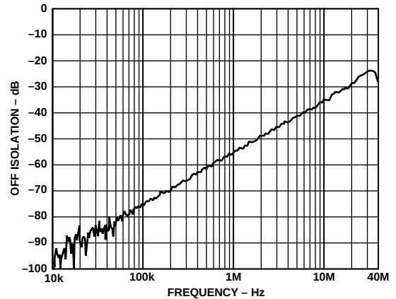
Figure 10. Off Isolation of the ADG467, V_{DD}/V_{SS} = 0 V and Input Signal Level of \pm 100 mV
