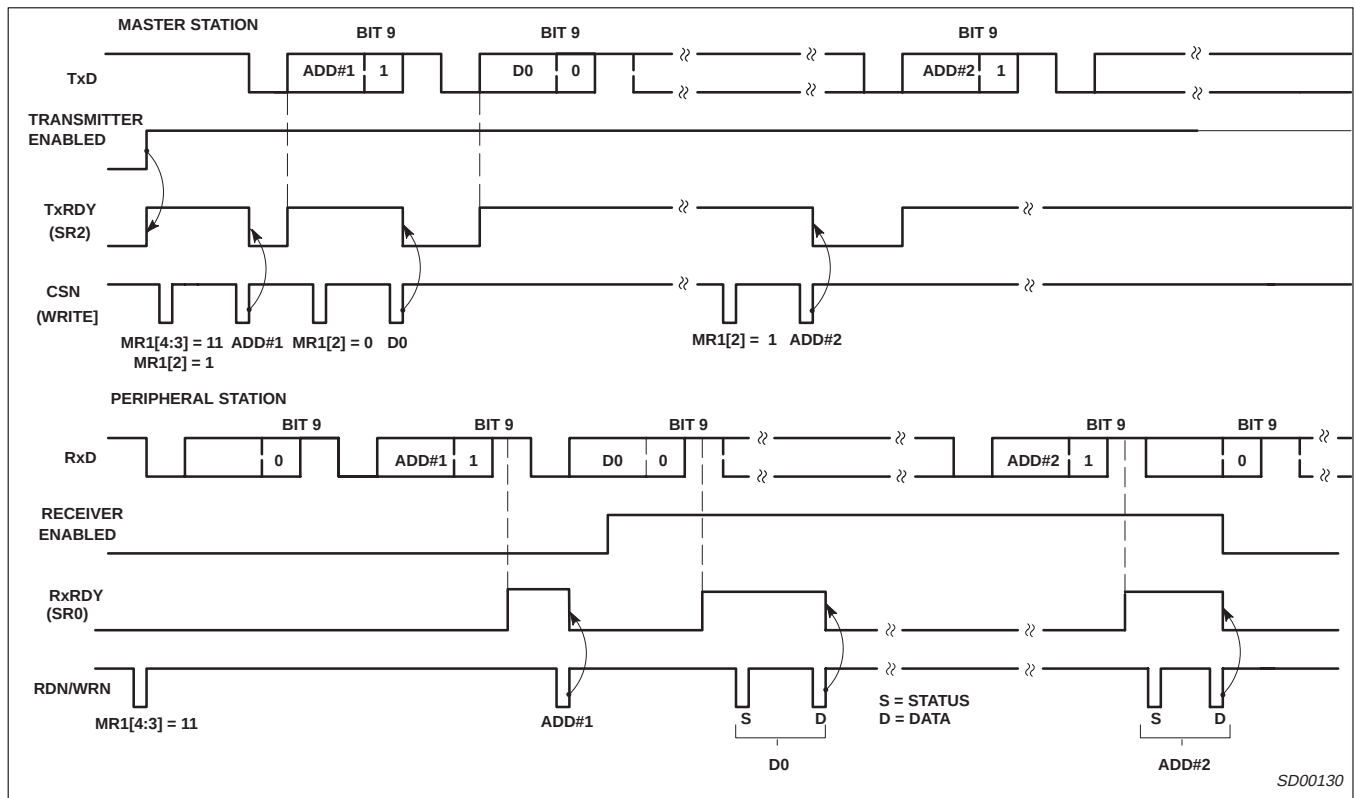
Figure 12. Wake-Up Mode
