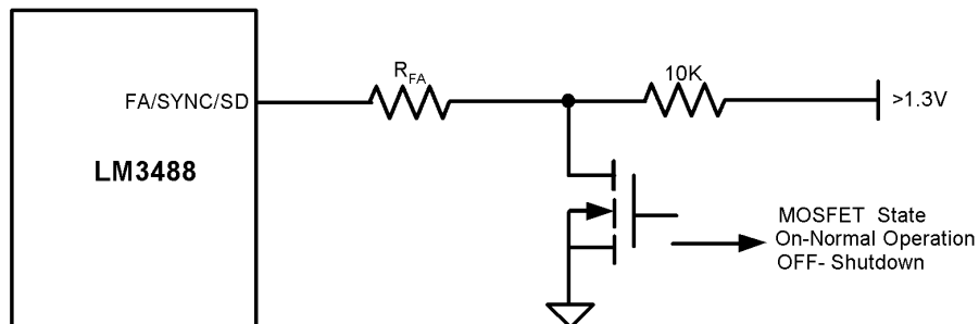
Figure 27. Shutdown Operation in Frequency Adjust Mode
