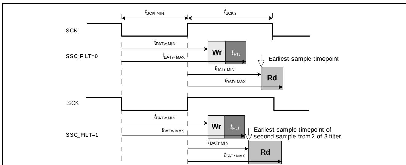
Figure 13 SSC Interface Timing Details - Worst-Case Specified Timing
