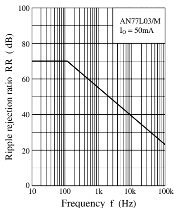
Ripple rejection ratio
