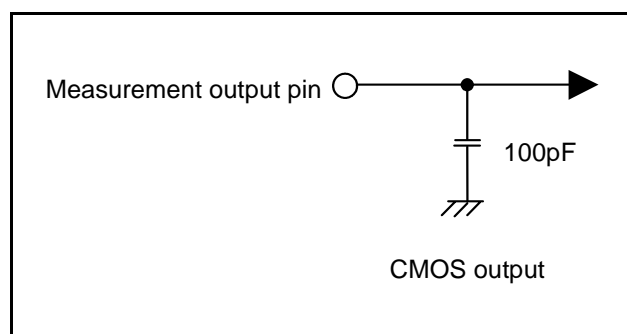
Fig 47. Circuit for measuring output switching characteristics
