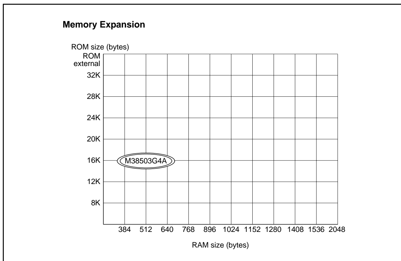
Fig 4. Memory expansion
