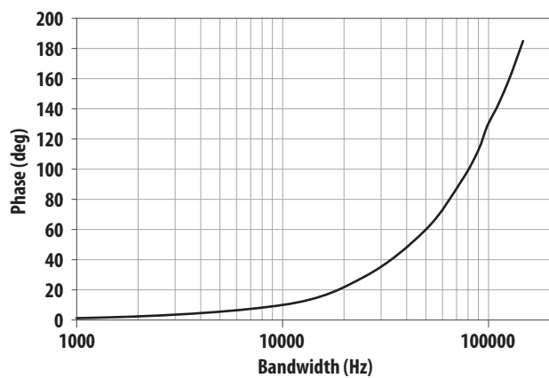
Figure 15. Phase Response
