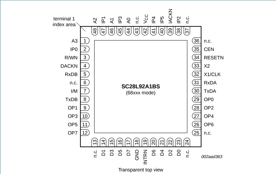
Fig 8. Pin configuration for HVQFN48; 68xxx mode
