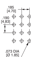
FOUR POLE
