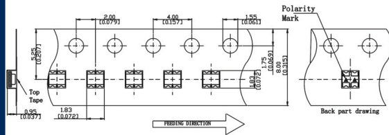
DIMENSIONS OF TAPE (UNIT:mm)
