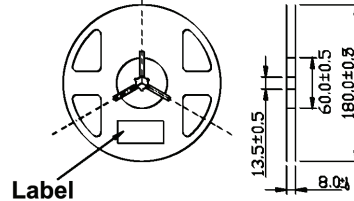
DIMENSIONS OF REEL (UNIT:mm)
