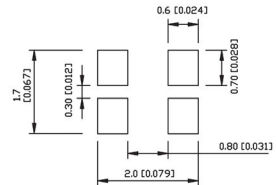
Recommended Soldering Pattern For Reflow Soldering
