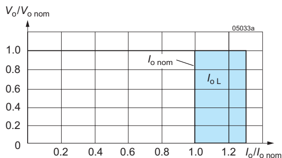
Fig. 6a Short-circuit behaviour V_o vs. I_o for regulators with V_{i \max} \leq 80 V
