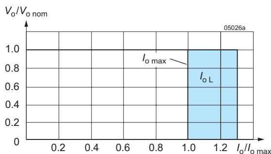
Fig. 6b Short-circuit behaviour V_o versus I_o for regulators with V_{i \max} = 144 V.
