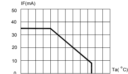
FIG.4b BLUE & GREEN MAXIMUM FORWARD DC CURRENT VS AMBIENT TEMPERATURE ( T_{jmax}=105^{\circ}\text{C} )
