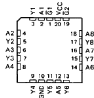
SN54ALS465A, SN54ALS466A . . . FK PACKAGE (TOP VIEW)
