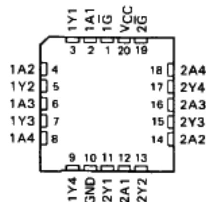
SN54ALS467A, SN54ALS468A . . . FK PACKAGE (TOP VIEW)
