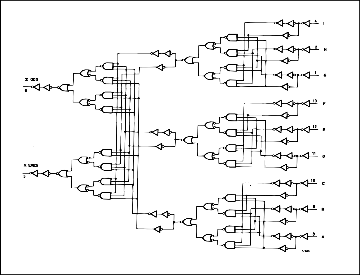
Figure 3: Logic Diagram
