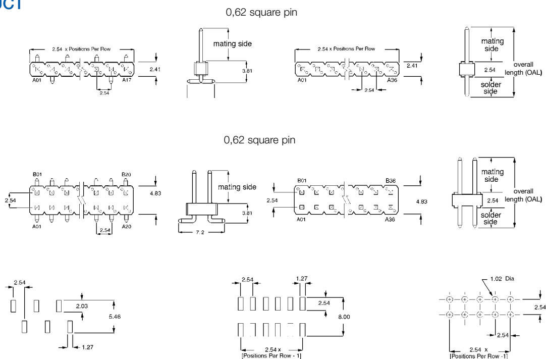
Recommended PCB layouts
