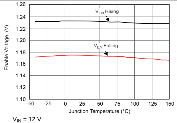
Figure 8. Enable-Pin Voltage vs Temperature
