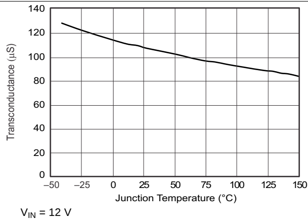
Figure 7. Error Amplifier Transconductance vs Temperature
