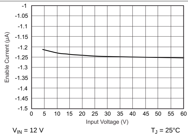
Figure 11. Enable-Pin Pullup Current vs Input Voltage
