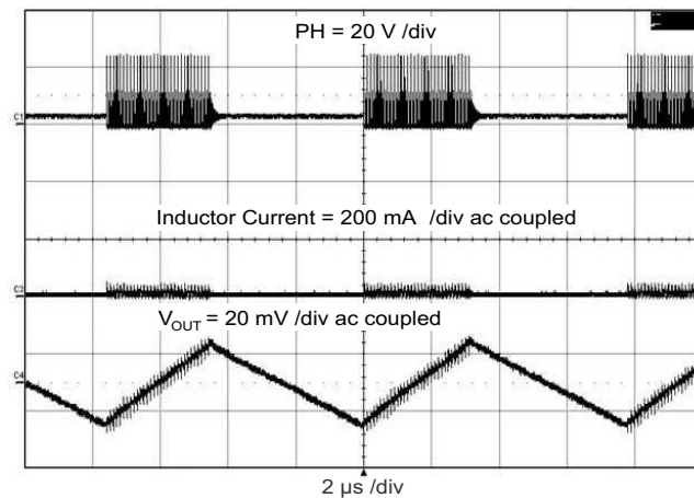
Figure 37. Output Ripple Skip
