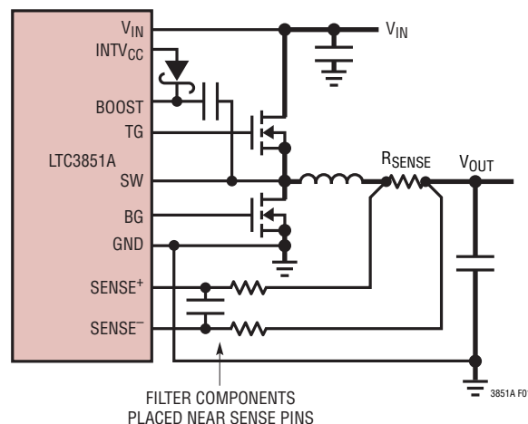
Figure 1. Using a Resistor to Sense Current with the LTC3851A
