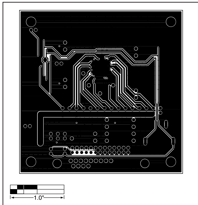
Figure 5. MAX2828/MAX2829 EV Kit PC Board Layout—Inner Layer 3
