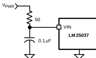
Figure 20. Input Transient Protection
