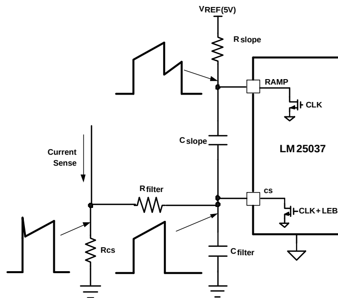
Figure 15. Current Mode Configuration With Slope Compensation
