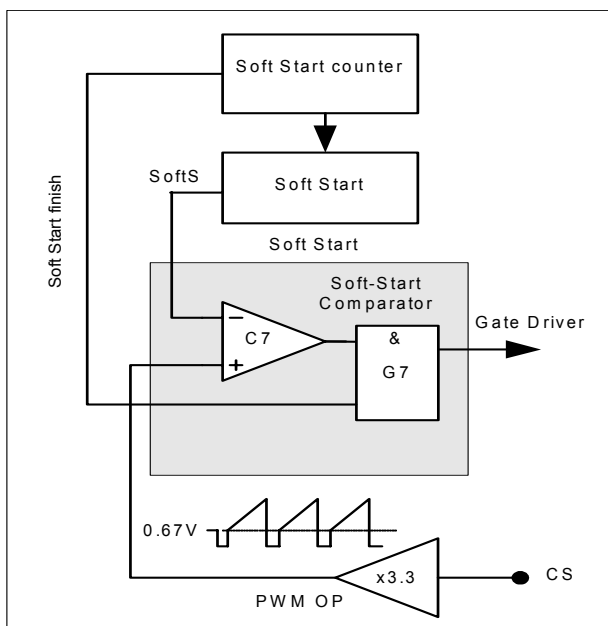
Figure 9 Soft Start
