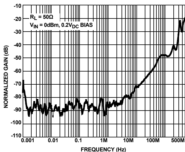
FIGURE 23. CROSSTALK
