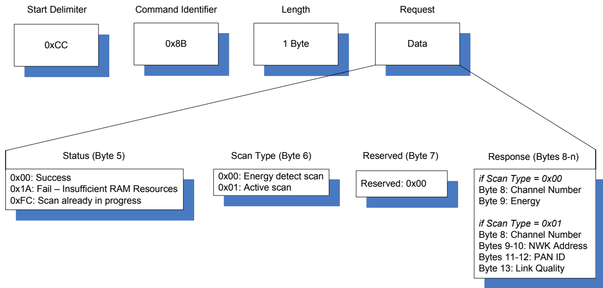
Figure 22: Perform Scan Response
