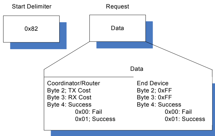
Figure 13: Send Data Complete packet format
