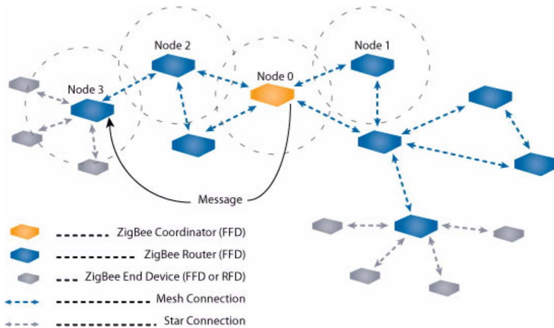
Figure 4: ZigBee AODV
