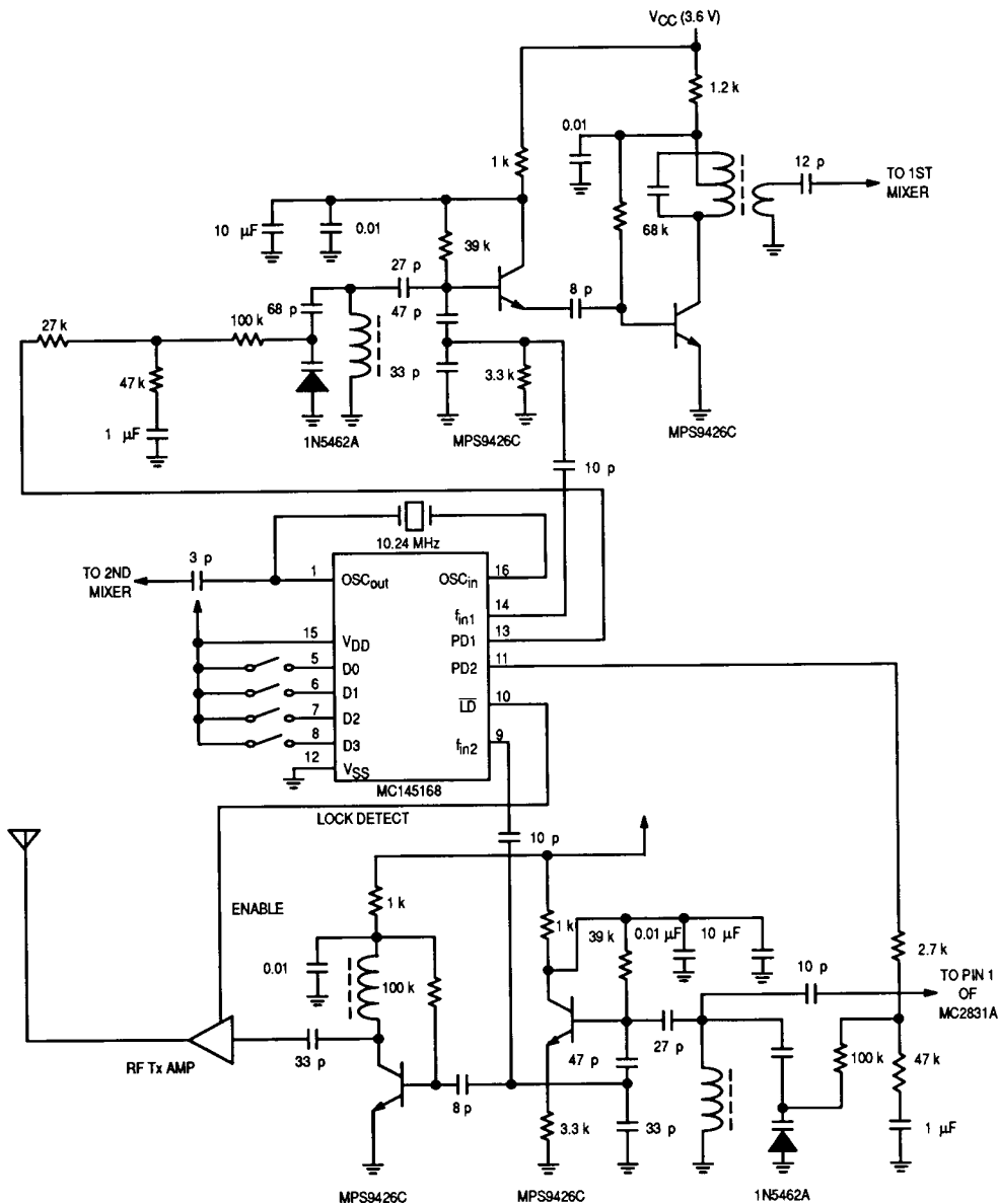
Figure 5. MC145168 Circuit Example
