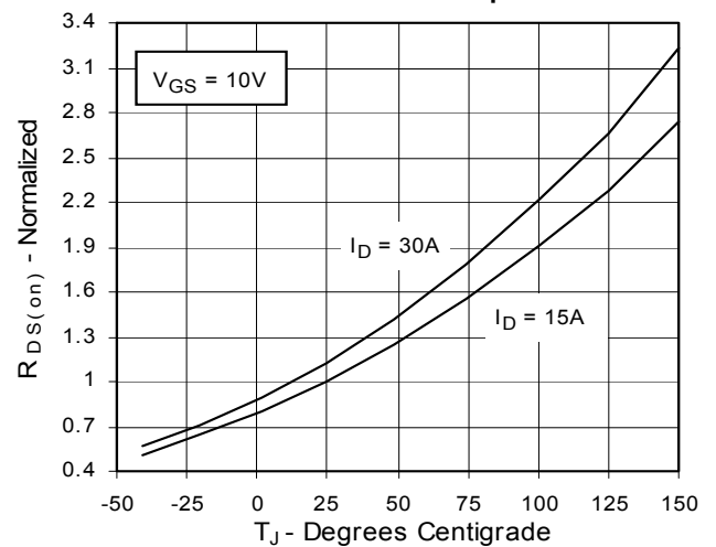
Fig. 4. R_{DS(on)} Normalized to I_D = 15\text{A} Value vs. Junction Temperature
