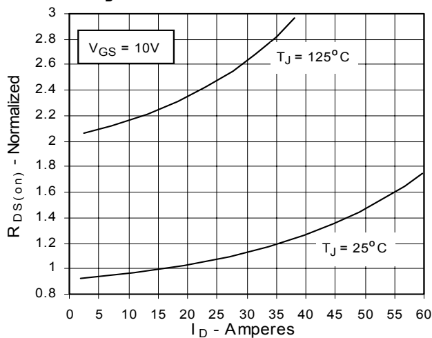
Fig. 5. R_{DS(on)} Normalized to I_D = 15\text{A} Value vs. Drain Current
