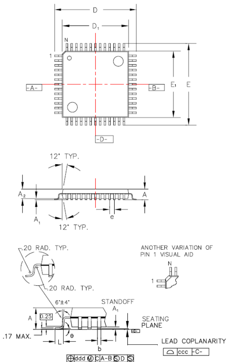
Figure D-1. Stellaris LM3S1850 100-Pin LQFP Package Dimensions
