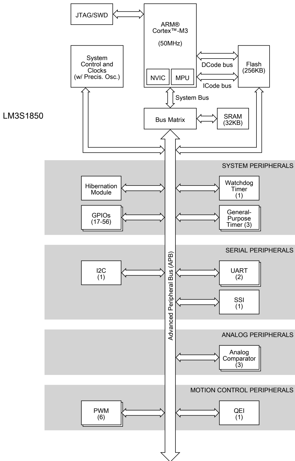
Figure 1-1. Stellaris LM3S1850 Microcontroller High-Level Block Diagram
