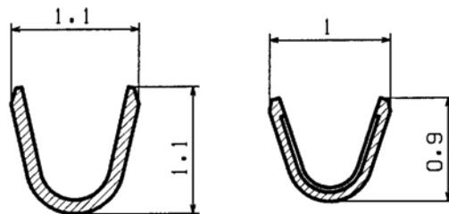
INSULATION BARREL Y-Y sec.
