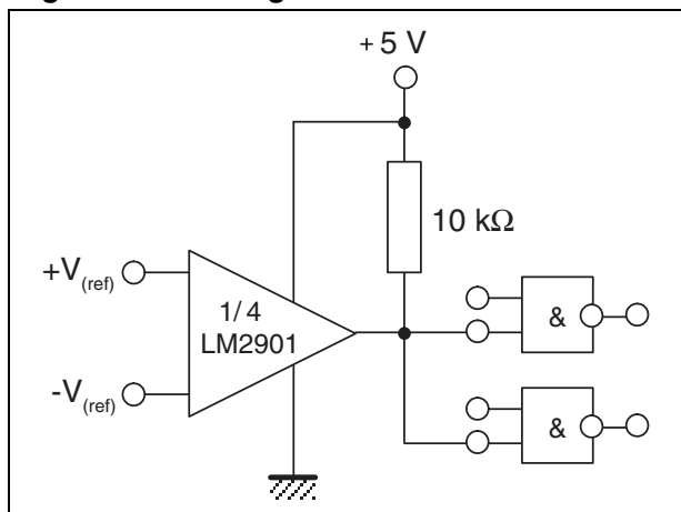
Figure 9. Driving TTL
