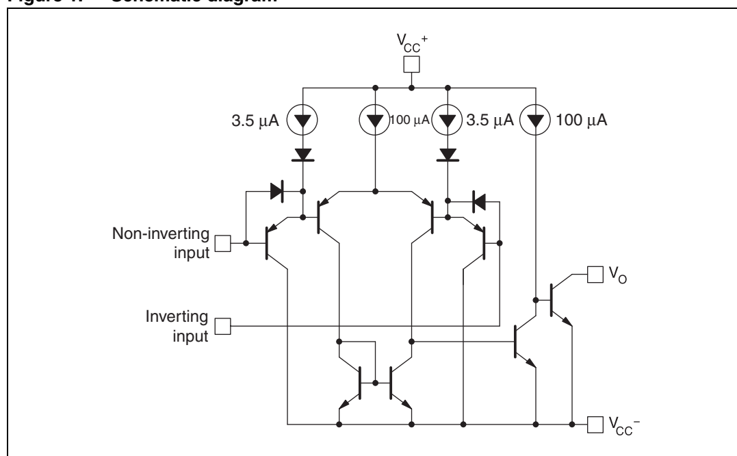
Figure 1. Schematic diagram
