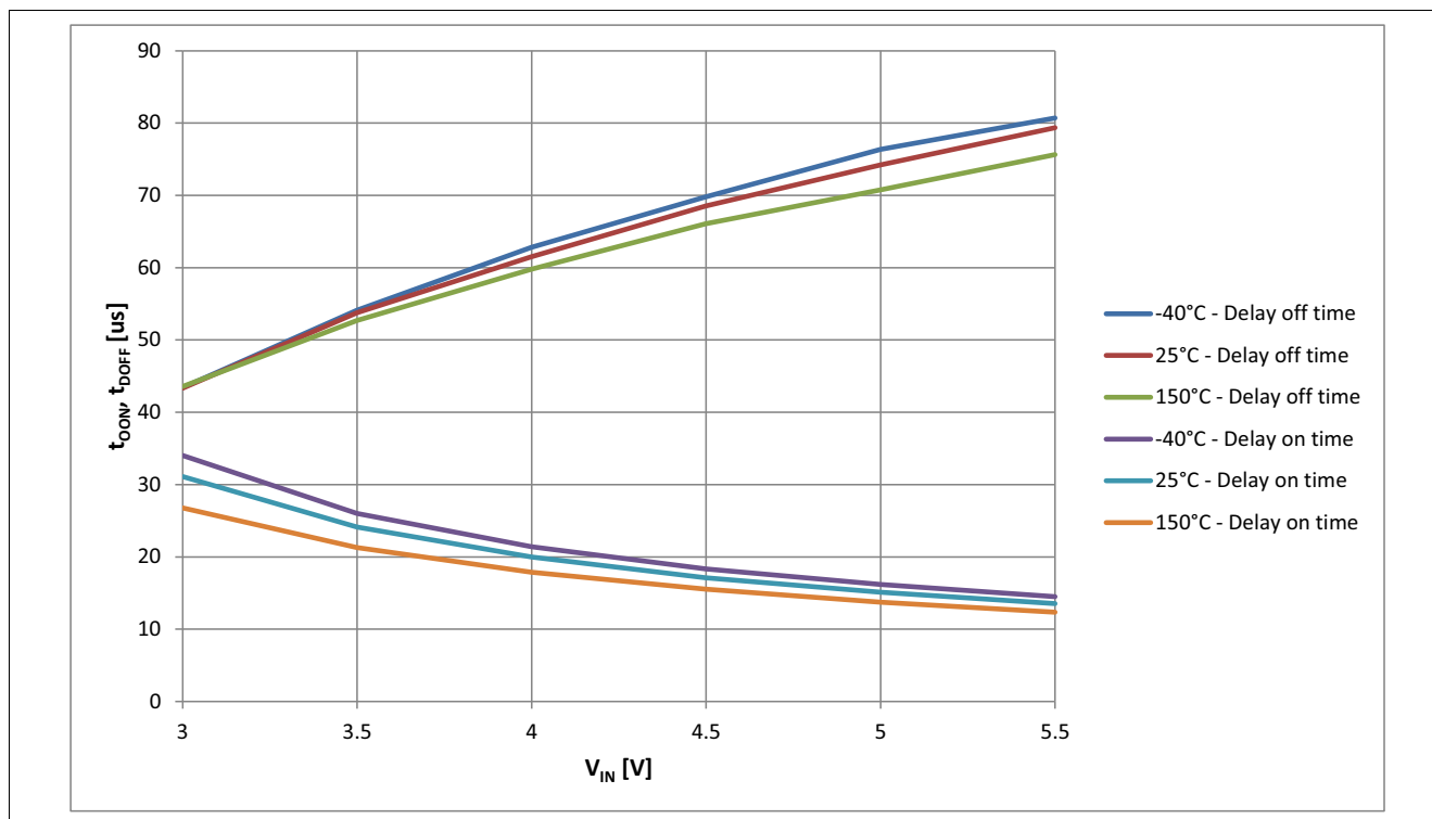
Figure 27 Typical t_{ON} , t_{OFF} vs V_{IN} @ T_J = -40 \dots 150^\circ C
