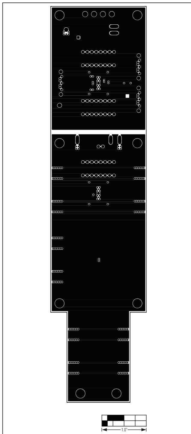
Figure 5. MAX4986 EV Kit PCB Layout—VCC Layer 3
