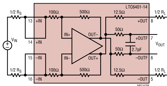
Figure 4. Calculate Differential Gain
