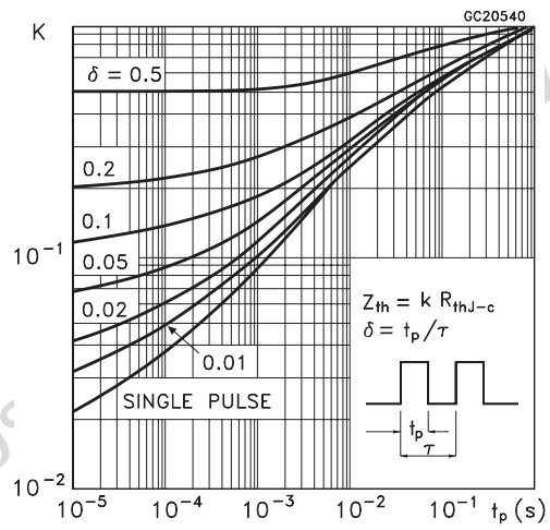
Figure 4. Thermal Impedance
