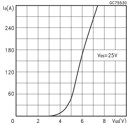
Figure 6. Transfer Characteristics
