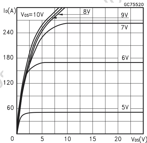
Figure 5. Output Characteristics
