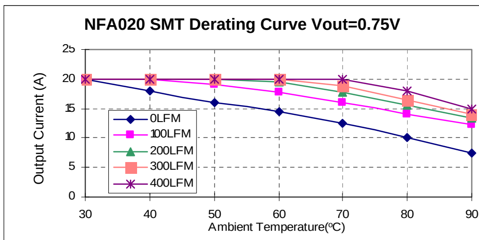
Fig. 2. SMT Derating of Output Current for 12Vin 0.75V Out.
