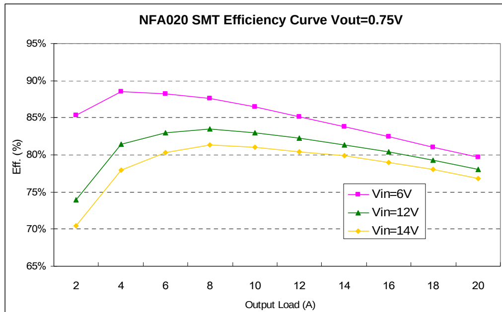
Fig 18. SMT Efficiency Curves for Vout=0.75V (25C)
