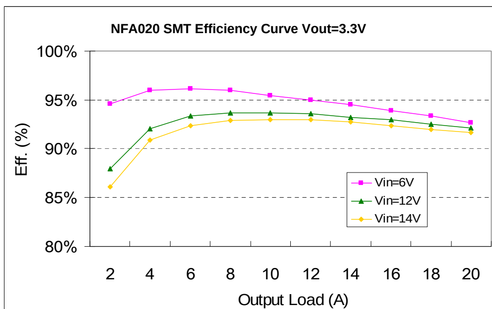
Fig 30. SMT Efficiency Curves for Vout=3.3V (25C)
