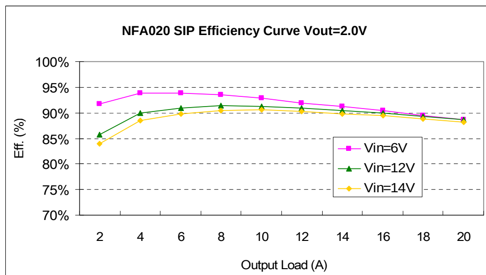
Fig 27. SIP Efficiency Curves for Vout=2.0V (25C)
