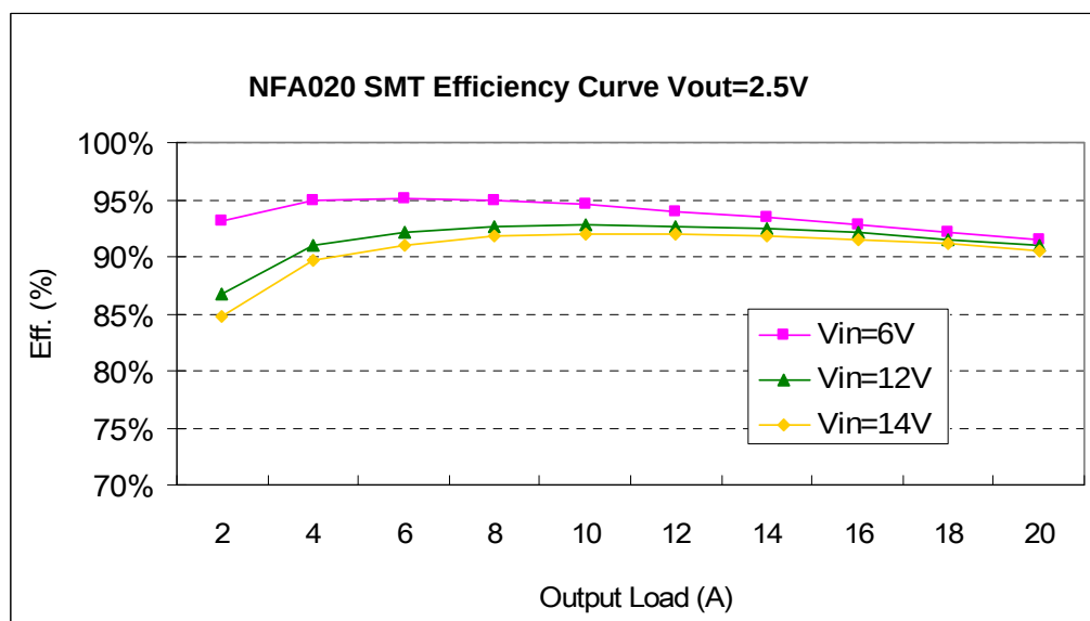
Fig 28. SMT Efficiency Curves for Vout=2.5V (25C)
