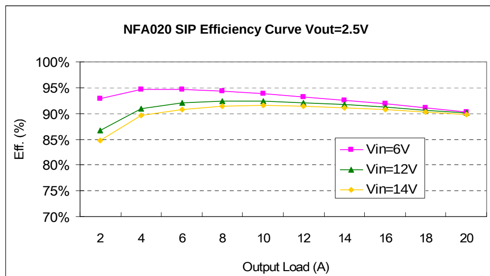
Fig 29. SIP Efficiency Curves for Vout=2.5V (25C)
