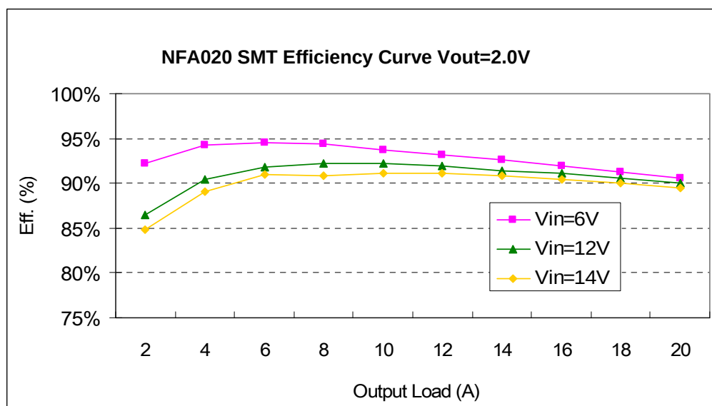
Fig 26. SMT Efficiency Curves for Vout=2.0V (25C)
