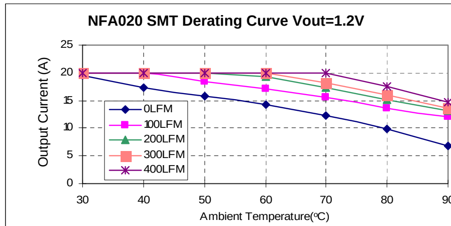
Fig 4. SMT Derating of Output Current for 12Vin 1.2V Out.
