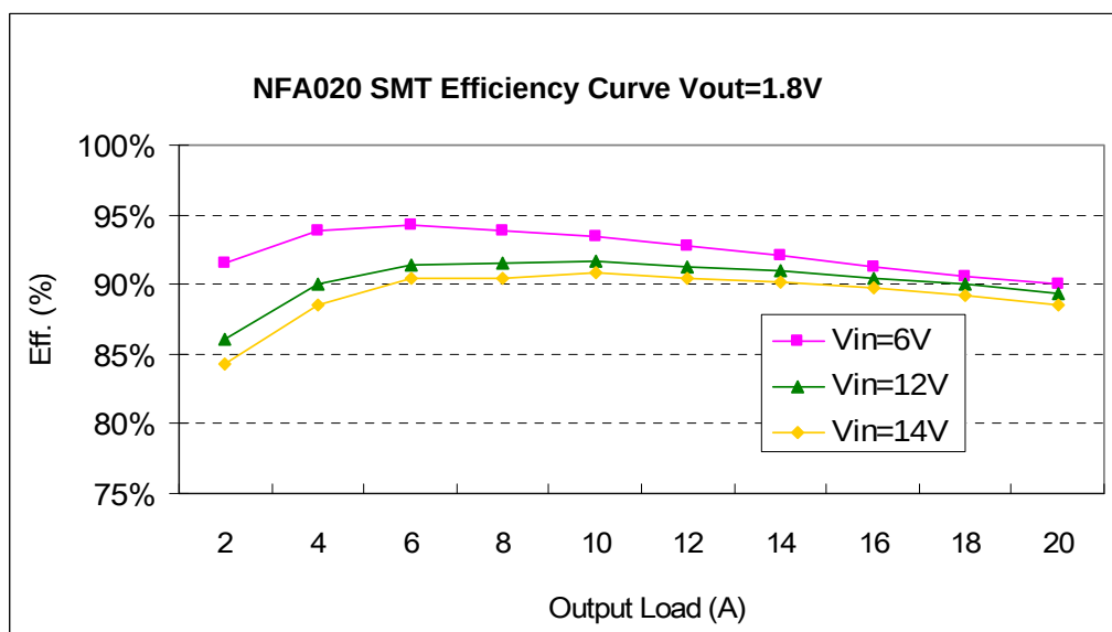
Fig 24. SMT Efficiency Curves for Vout=1.8V (25C)
