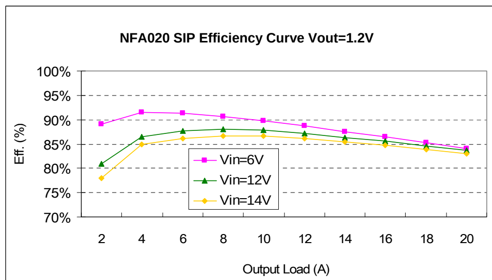
Fig 21. SIP Efficiency Curves for Vout=1.2V (25C)
