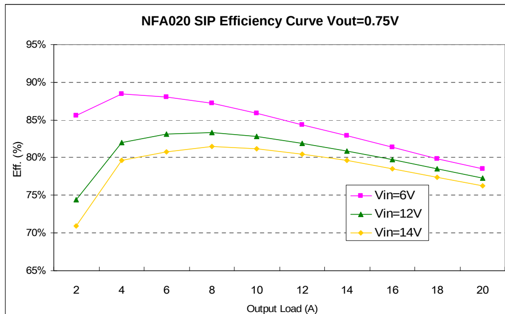
Fig 19. SIP Efficiency Curves for Vout=0.75V (25C)
