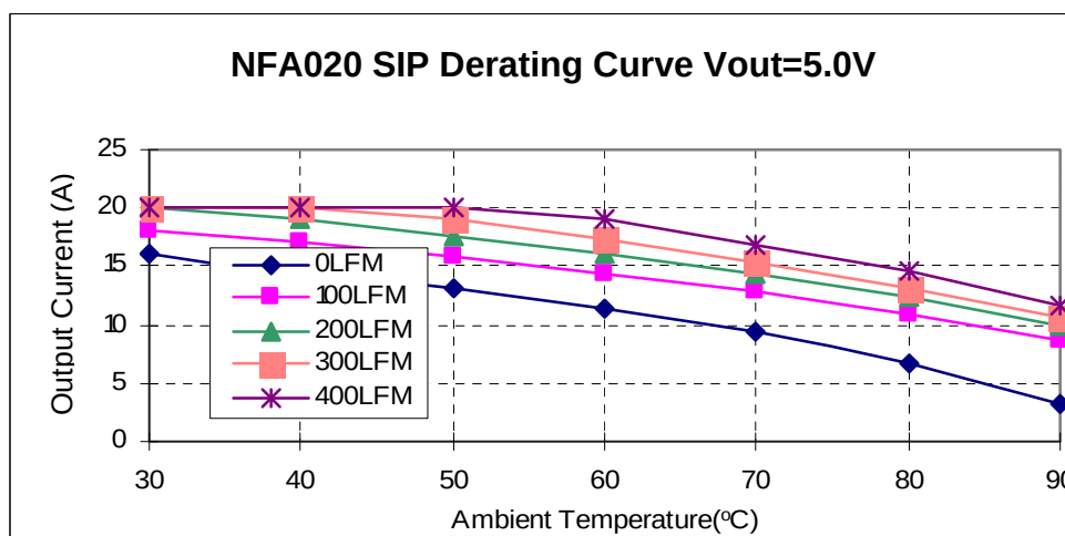
Fig 17. SIP Derating of Output Current for 12Vin 5.0V Out.
