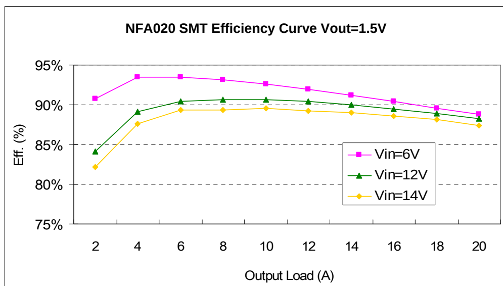
Fig 22. SMT Efficiency Curves for Vout=1.5V (25C)
