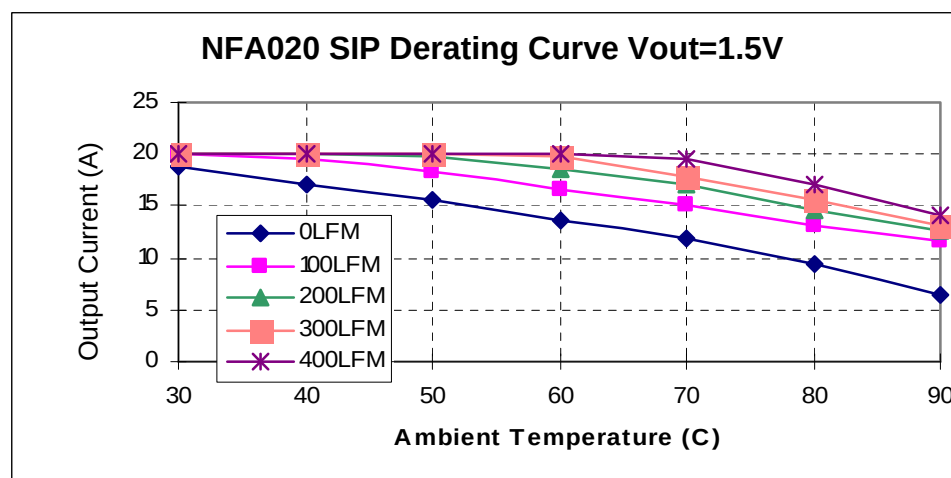
Fig 7. SIP Derating of Output Current for 12Vin 1.5V Out.
