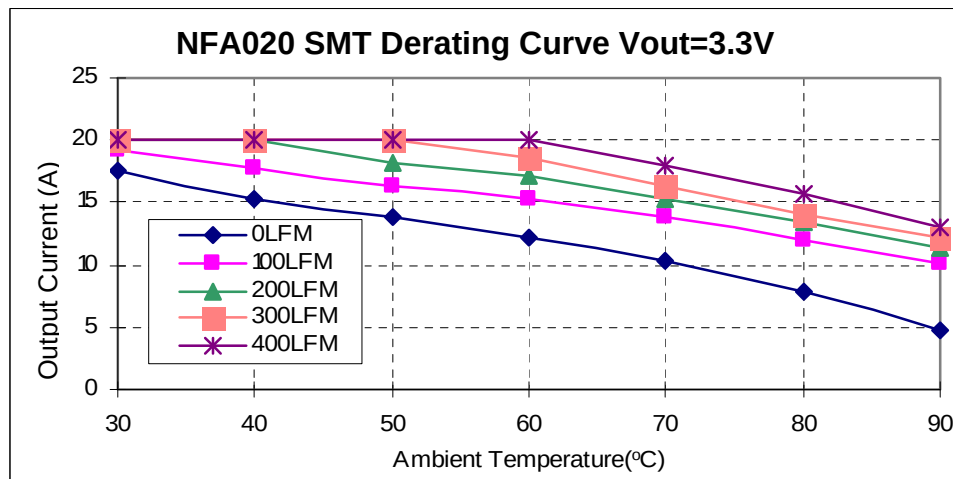
Fig. 14. SMT Derating of Output Current for 12Vin 3.3V Out.
