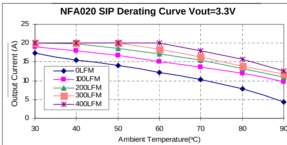
Fig. 15. SIP Derating of Output Current for 12Vin 3.3V Out.
