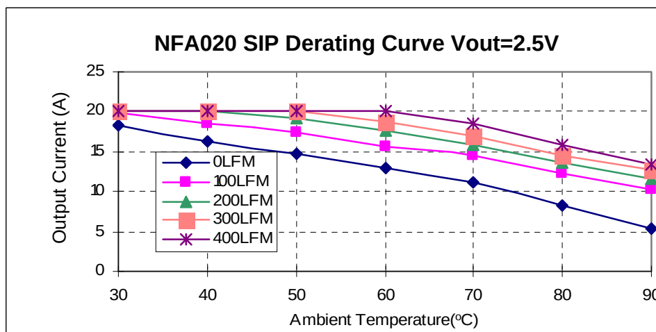
Fig 13. SIP Derating of Output Current for 12Vin 2.5V Out.
