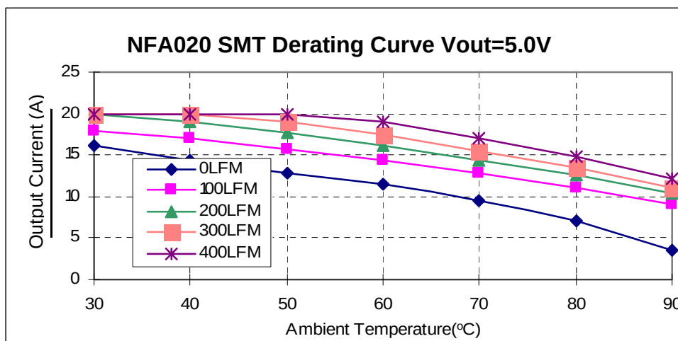
Fig. 16. SMT Derating of Output Current for 12Vin 5.0V Out
