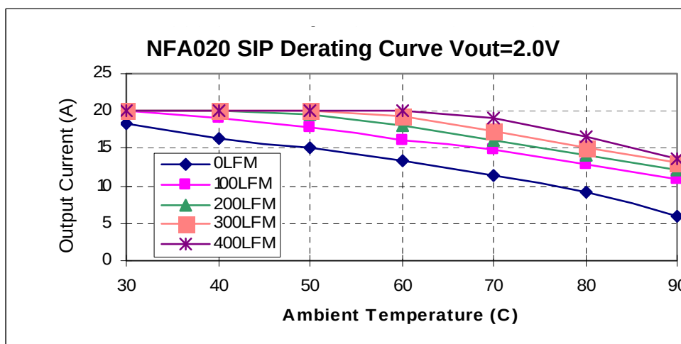
Fig 11. SIP Derating of Output Current for 12Vin 2.0V Out.
