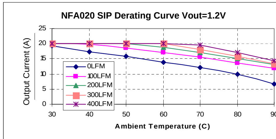
Fig 5. SIP Derating of Output Current for 12Vin 1.2V Out.
