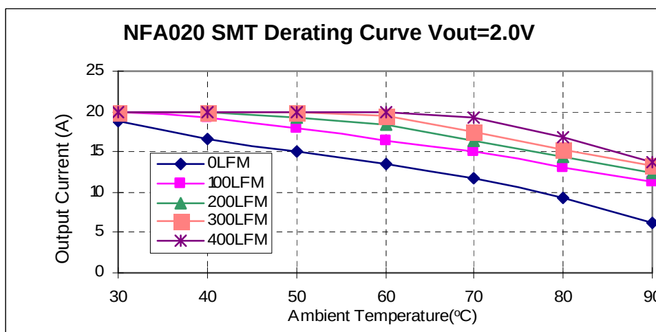
Fig 10. SMT Derating of Output Current for 12Vin 2.0V Out.
