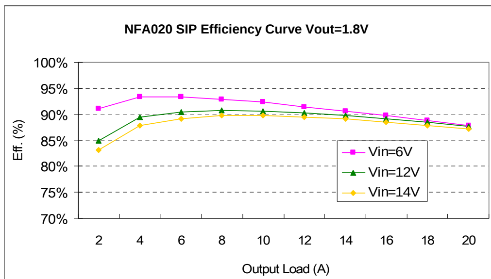
Fig 25. SIP Efficiency Curves for Vout=1.8V (25C)
