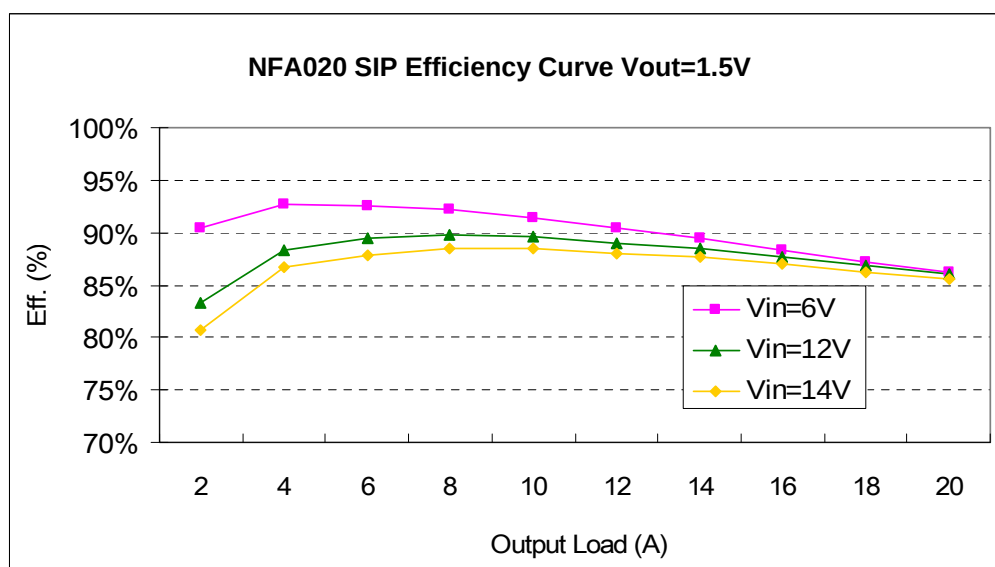
Fig 23. SIP Efficiency Curves for Vout=1.5V (25C)
