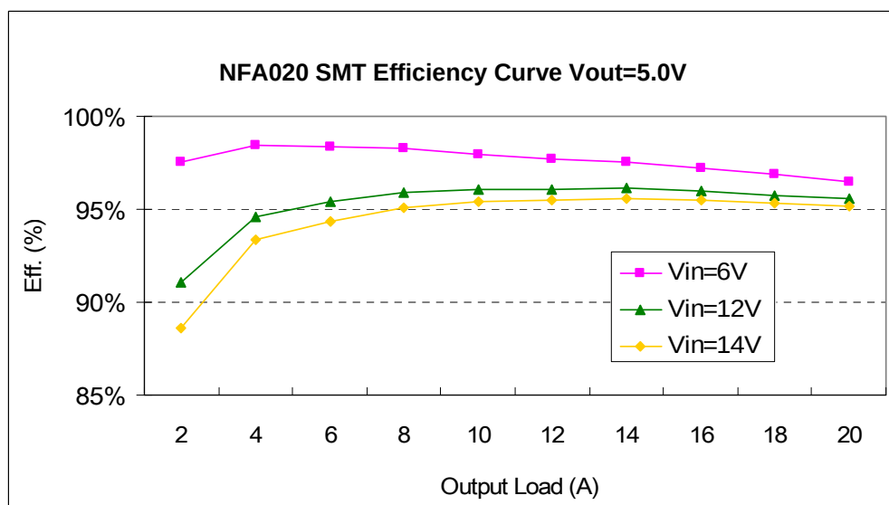
Fig 32. SMT Efficiency Curves for Vout=5.0V (25C)
