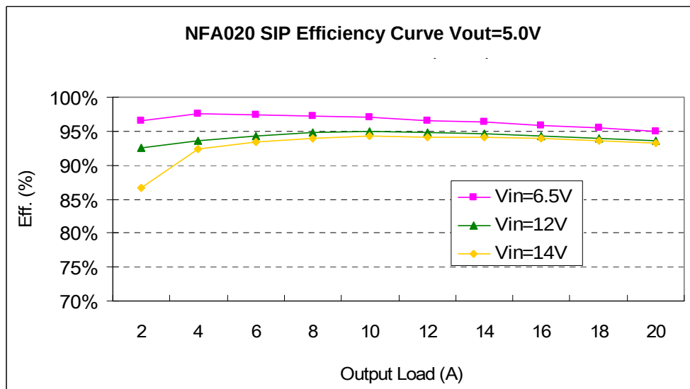
Fig 33. SIP Efficiency Curves for Vout=5.0V (25C)
