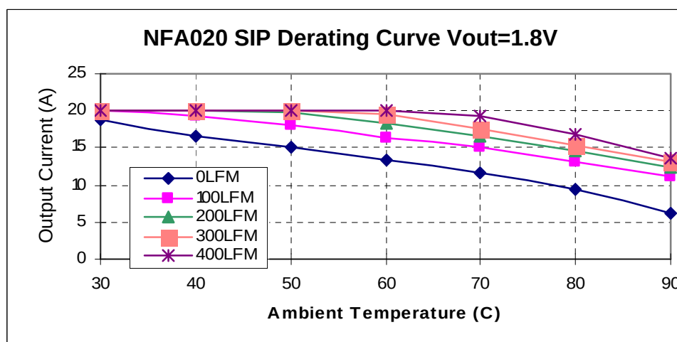
Fig 9. SIP Derating of Output Current for 12Vin 1.8V Out.
