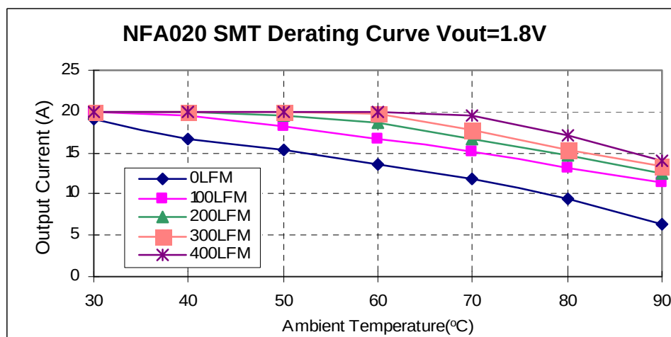
Fig 8. SMT Derating of Output Current for 12Vin 1.8V Out.
