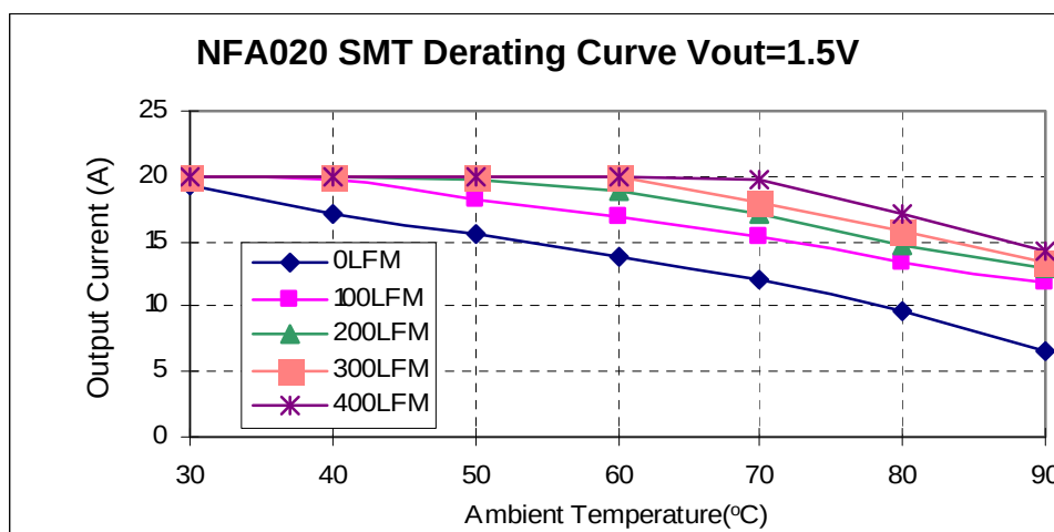
Fig 6. SMT Derating of Output Current for 12Vin 1.5V Out.
