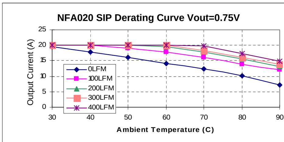
Fig. 3. SIP Derating of Output Current for 12Vin 0.75V Out.
