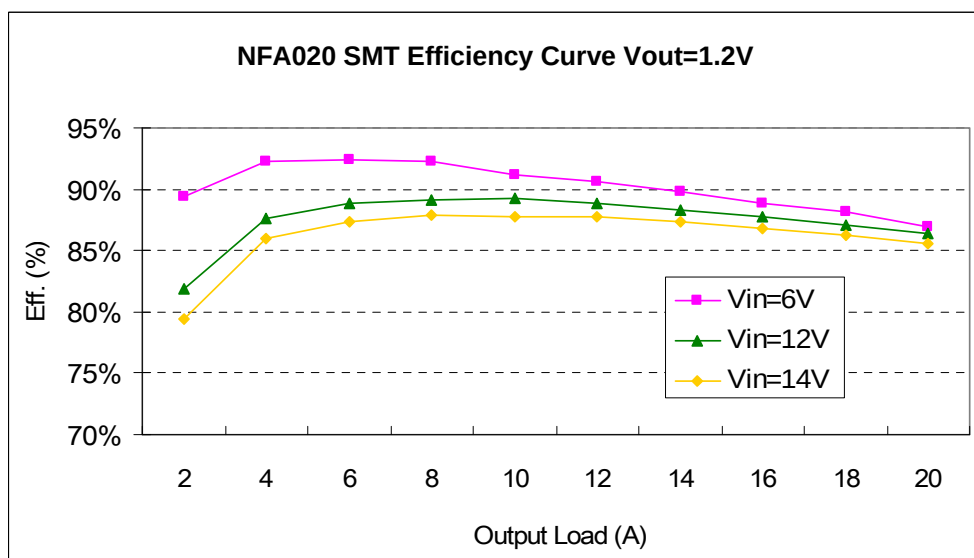
Fig 20. SMT Efficiency Curves for Vout=1.2V (25C)
