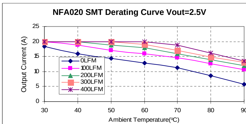
Fig 12. SMT Derating of Output Current for 12Vin 2.5V Out.
