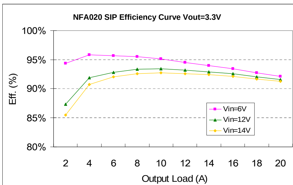
Fig 31. SIP Efficiency Curves for Vout=3.3V (25C)
