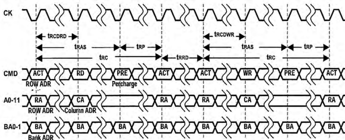
Figure 3. Bank Activate Read or Write Command Timing
