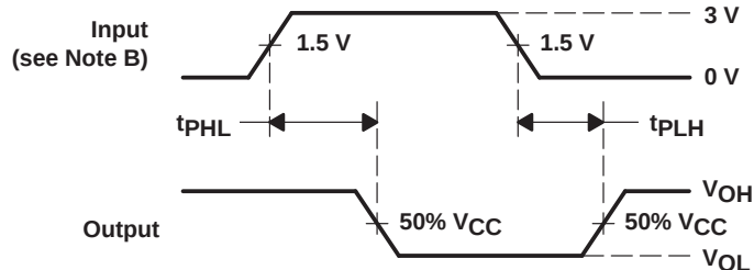
VOLTAGE WAVEFORMS
