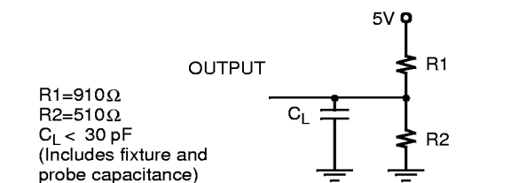
(a) TTL AC Test Load [6]
