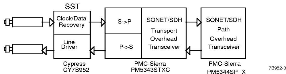
Figure 1. SONET/SDH Overhead Processing Application
