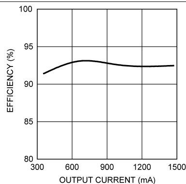
Figure 2. Efficiency Vs. Output Current (1)
