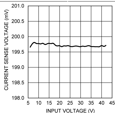
Figure 4. V_{REF} vs V_{IN} , LM3406
