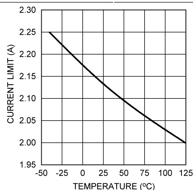
Figure 6. Current Limit vs Temperature
