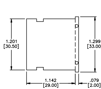
DPS910A2 Spacer
