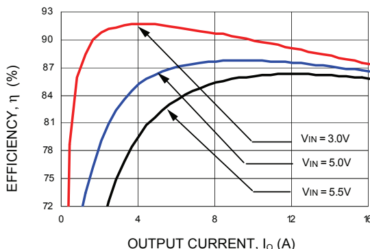
Figure 2. Converter Efficiency versus Output Current (V out = 1.2Vdc).
