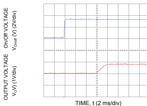
Figure 17 Typical Start-Up Using Remote On/Off with Prebias ( V_{in} = 3.3 Vdc, V_o = 1.8 Vdc, I_o = 1.0 A, V_{bias} = 1.0 Vdc).
