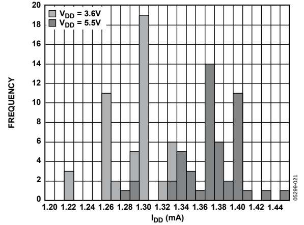
Figure 21. I_{DD} Histogram with External Reference
