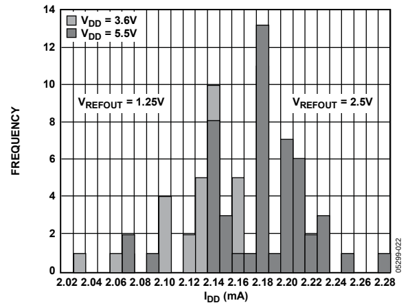
Figure 22. I_{DD} Histogram with Internal Reference
