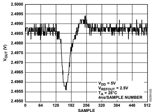
Figure 35. Analog Crosstalk
