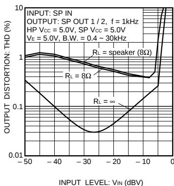
Fig. 11 SP AMP input level vs. output distortion
