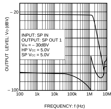
Fig.10 SP AMP frequency characteristics
