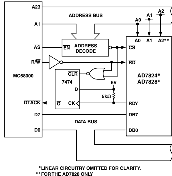
Figure 17. AD7824/AD7828–MC68000 Interface
