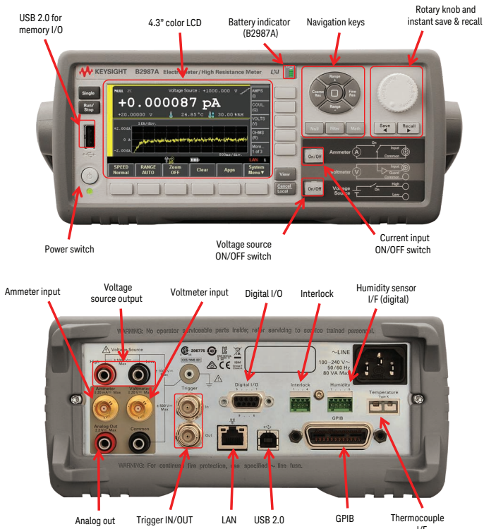
B2985A, B2987A Electrometer/High Resistance Meter
