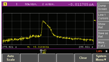
Time domain view (Roll View)
