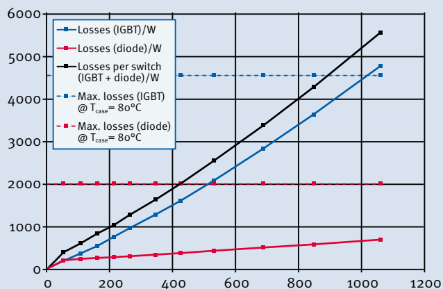
Average losses for sinusoidal output current at 400 Hz switching frequency
