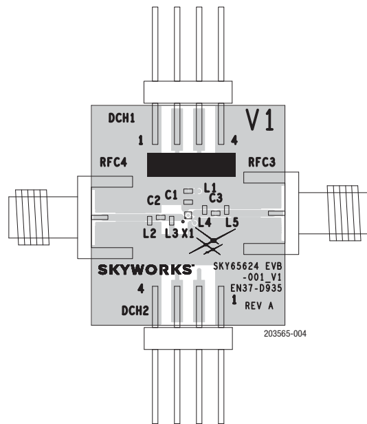
Figure 4. SKY65623-682LF Evaluation Board Assembly Diagram
