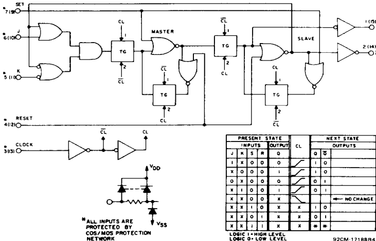
Fig. 2 - Logic diagram & truth table for CD4027A (one of two identical J-K flip flops).
