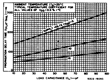
Fig. 6 - Typical propagation delay time vs. C L .
