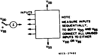
Fig. 11 — Input leakage current test circuit.
