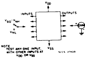
Fig. 10 — Noise immunity test circuit.
