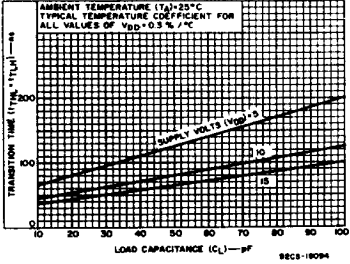
Fig. 7 — Typical transition time vs. C_L .
