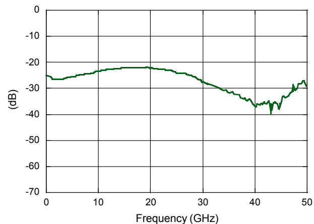
Output Return Loss @ -5 V (Insertion Loss State)
